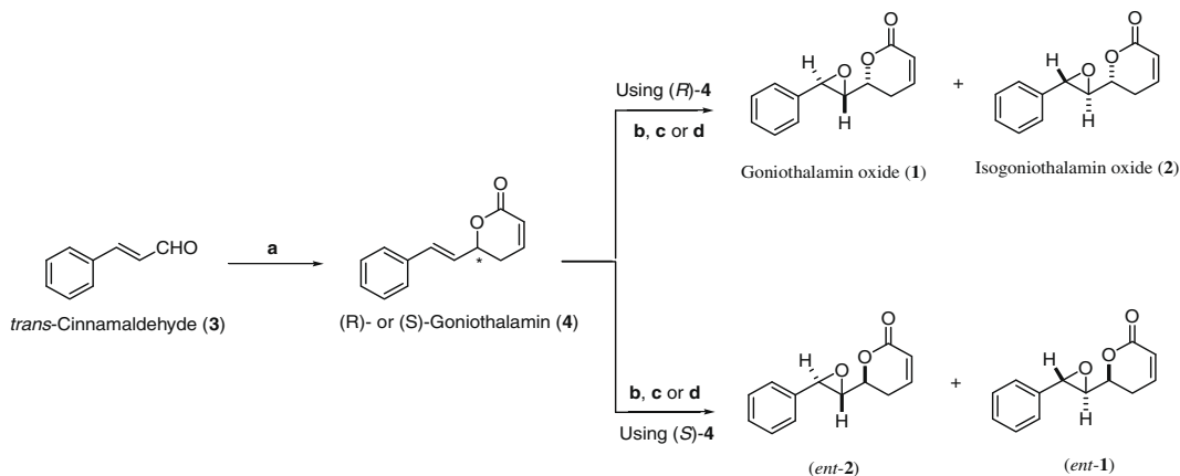
Scheme 1. Synthesis of goniiothalamine oxide ( 1 ), ent - 1 , isogoniiothalamine oxide ( 2 ), and ent - 2 from ( R )- or ( S )-goniiothalamine ( 4 ). Conditions: (a) see Ref. [16–19]; (b) mCPBA (70%), \text{CH}_2\text{Cl}_2 , room temperature, 5 h (61–64%); (c) ( R,R )-Jacobsen, \text{CH}_2\text{Cl}_2 ; \text{Na}_2\text{HPO}_4 (0.05 mol/L) and commercial household bleach, pH 11.3 at 0 ^\circ\text{C} , then room temperature, 5 h (49–52%); (d) ( S,S )-Jacobsen, \text{CH}_2\text{Cl}_2 ; \text{Na}_2\text{HPO}_4 (0.05 mol/L) and commercial household bleach, pH 11.3 at 0 ^\circ\text{C} , then room temperature, 5 h (49–52%).
