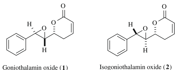
Fig. 1. Structures of goniiothalamin oxide ( 1 ) and isogoniiothalamin oxide ( 2 ).
